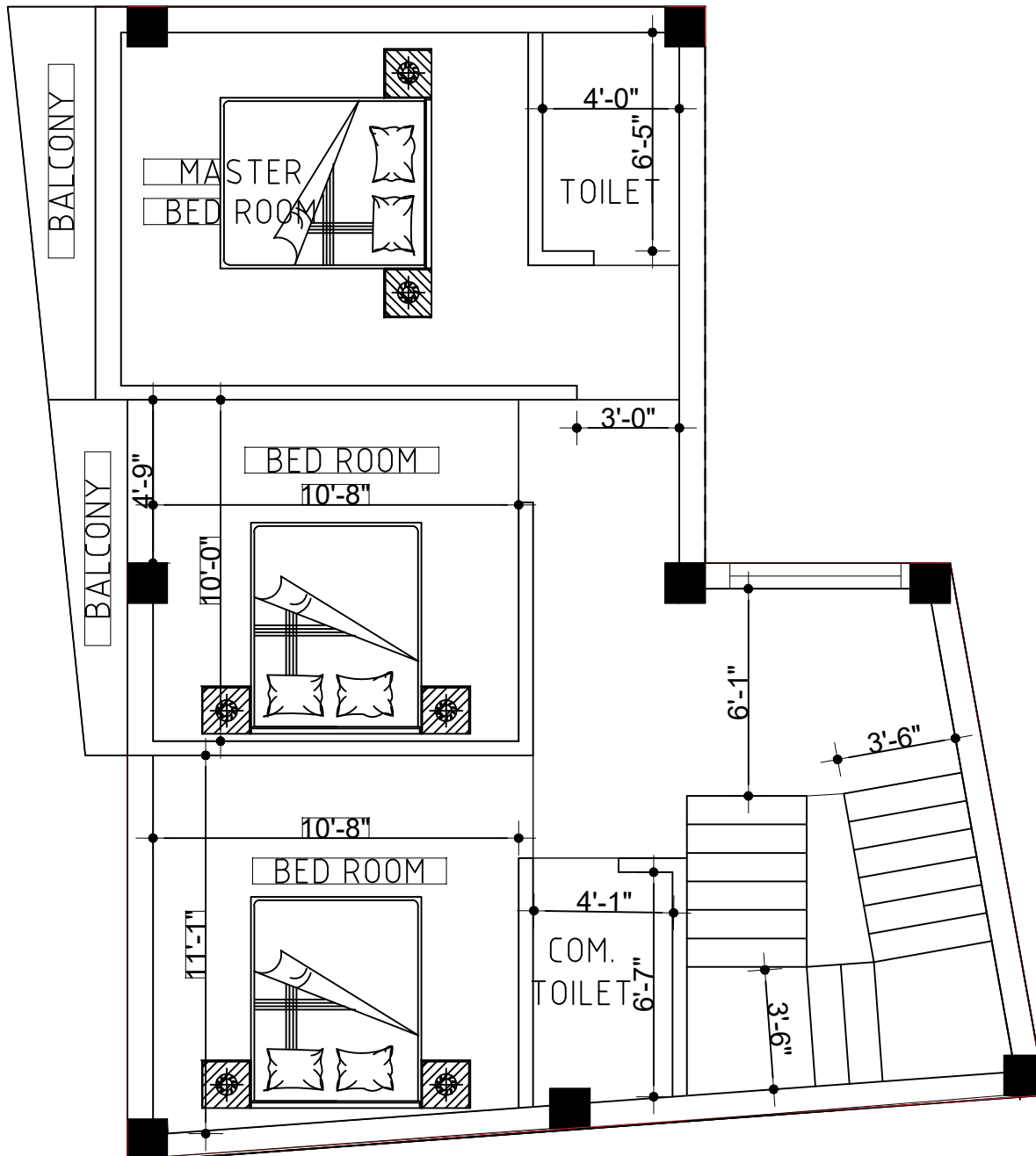
FIRST FLOOR PLAN -1 FLOOR AREA =713 Sq.ft
